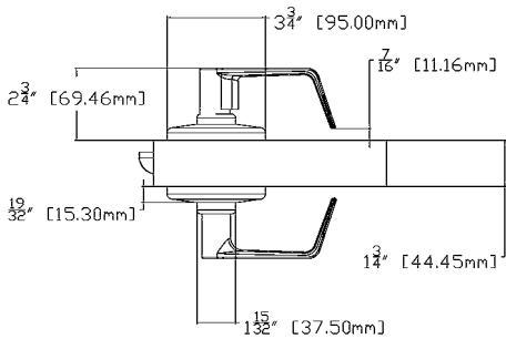
CE-R Dimensions
